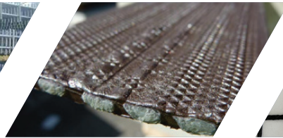
Geostrip reinforcement
